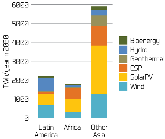
Figure 7 2030 generation by technology under 100% renewables scenario
