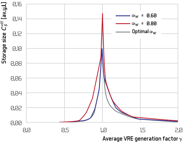
Figure 3 Storage results from Rasmussen et al. \alpha_w refers to the proportion from wind of total renewable generation, with solar as the remainder.
