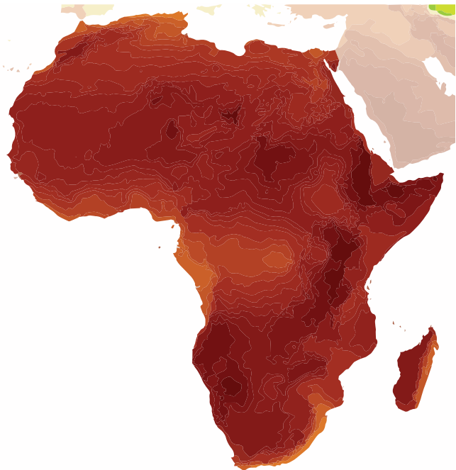
Figure 8 Solar energy resource (GHI) for Africa. Sources: see note 28
