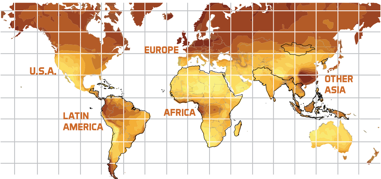
Figure 6 Solar Direct Normal Irradiation (DNI) resource. Dark colours are lowest resource, light is highest. World regions relevant to this study outlined in black. Sources: see note 19
